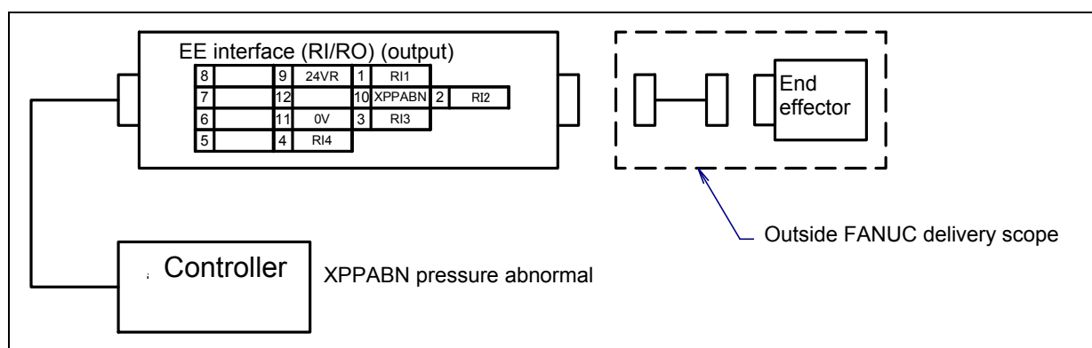
Fig. 5.2 (d) EE (RI/RO) interface (When A05B-1118-H202,H252 is specified)
