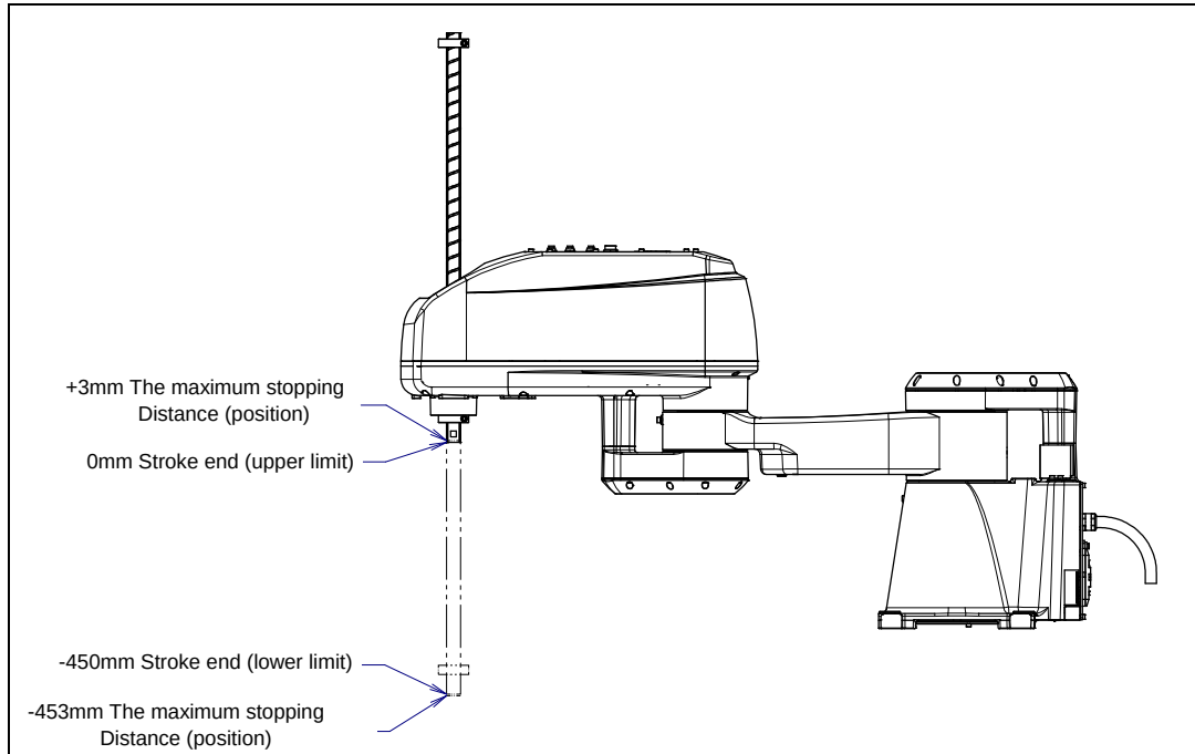
Fig. 3.3 (e) J3-axis motion limit (450mm stroke)
