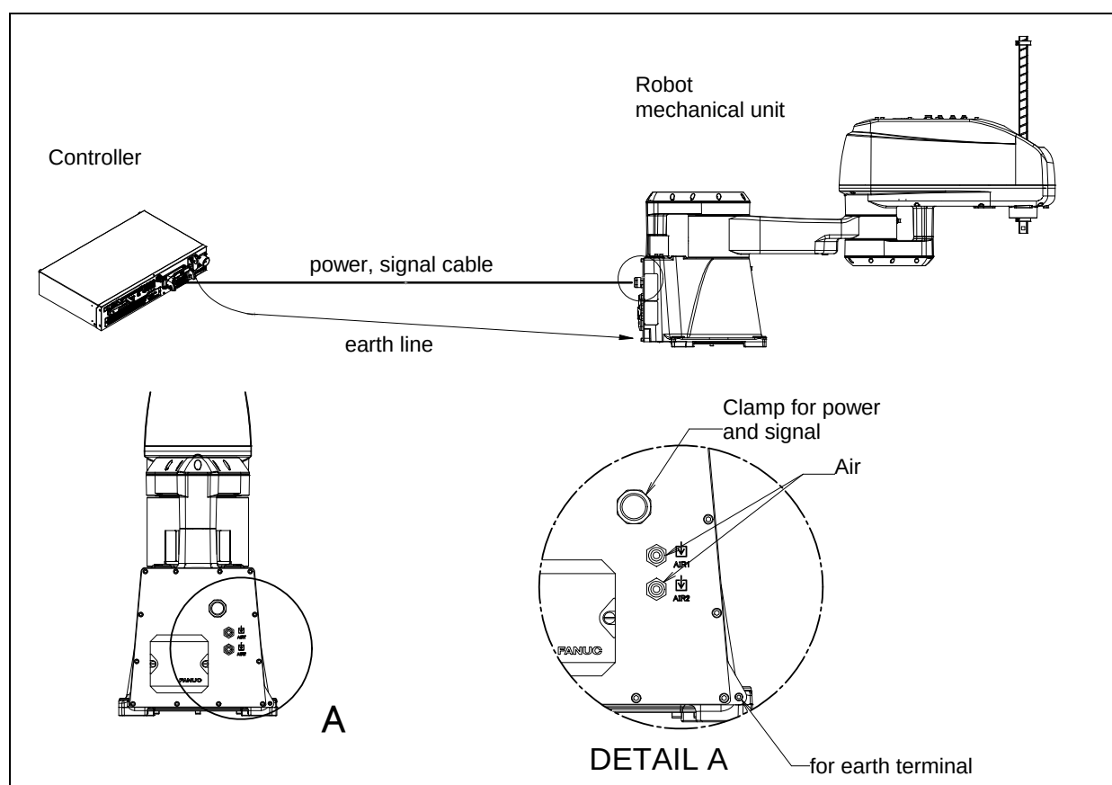
Fig. 2.1 (a) Cable connection (back side connector panel)
