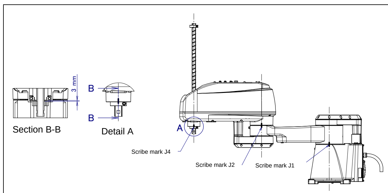
Fig. 8.3 (a) Marking position
