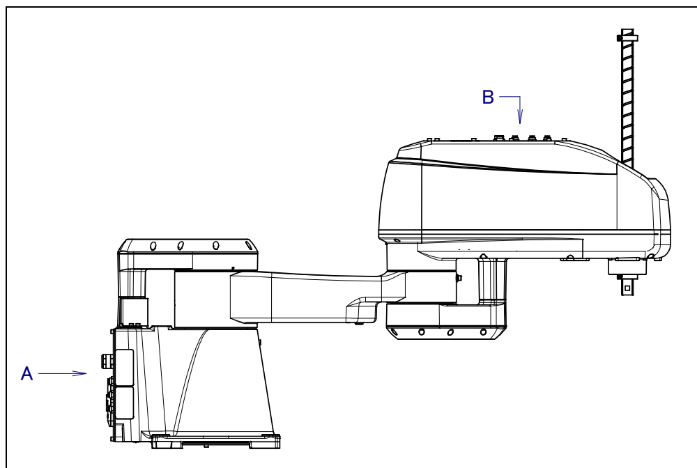
Fig. 5.2 (a) Air supply and EE (RI/RO) interface position
