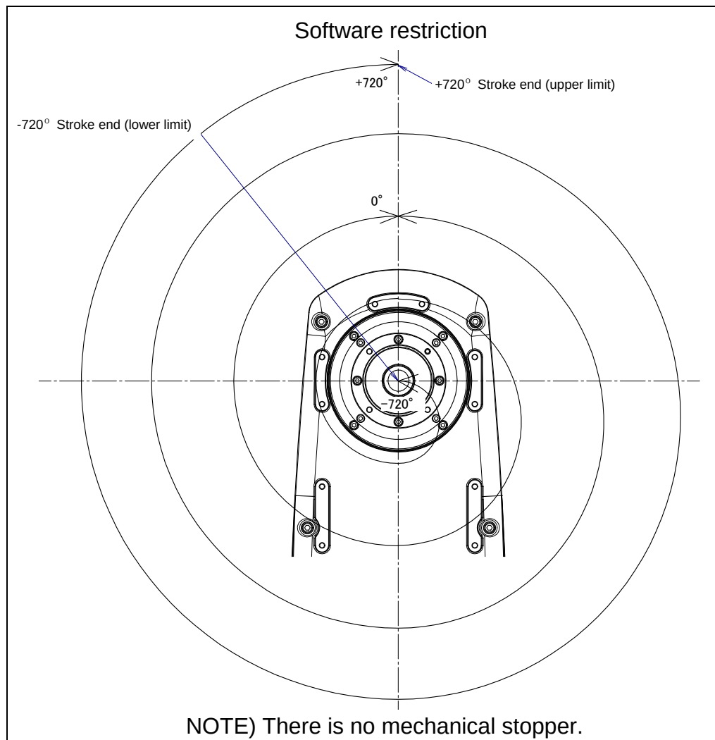
Fig. 3.3 (f) J4-axis motion limit
