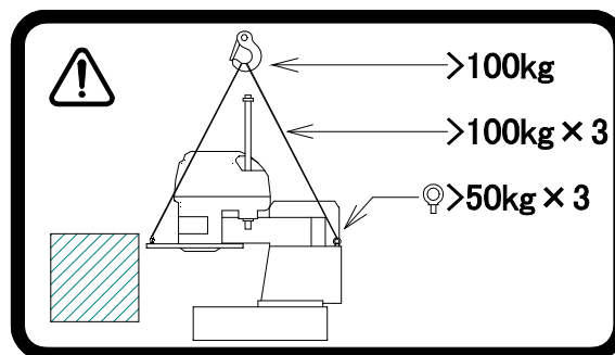
Fig. 5 (a) Transportation label
