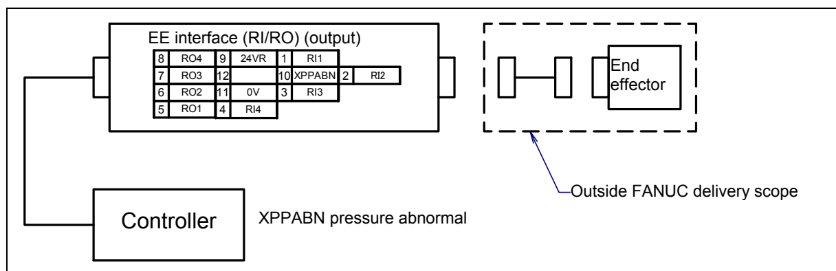
Fig. 5.2 (c) EE (RI/RO) interface (When A05B-1118-H201,H251 is specified)
