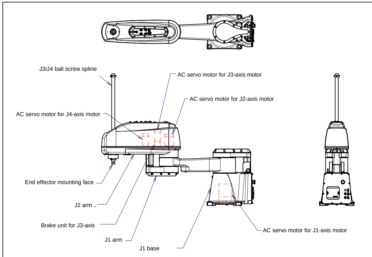
Fig. 3.1 (a) Mechanical unit configuration
