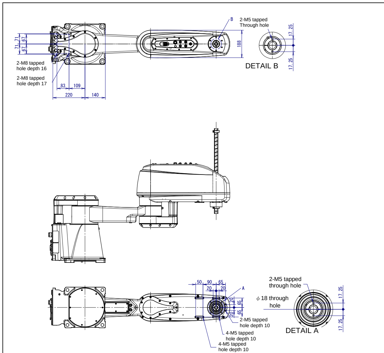
Fig. 4.2 (a) Equipment mounting faces (SR-12iA)
