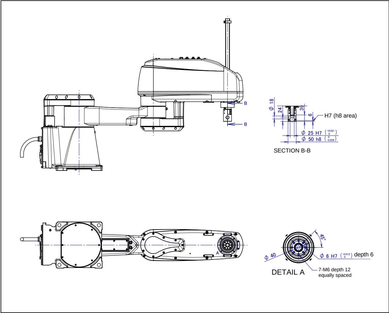
Fig. 4.2 (b) Equipment mounting faces (SR-12iA, SR-20iA) (tool flange option)
