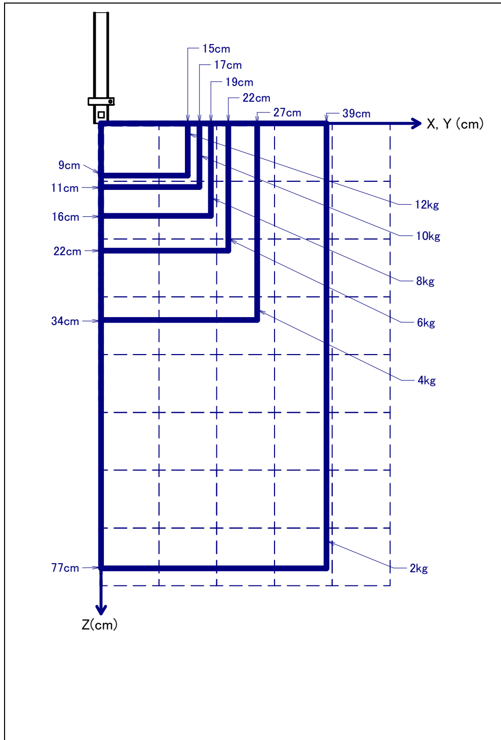
Fig. 3.4 (a) Wrist load diagram (SR-12iA)
