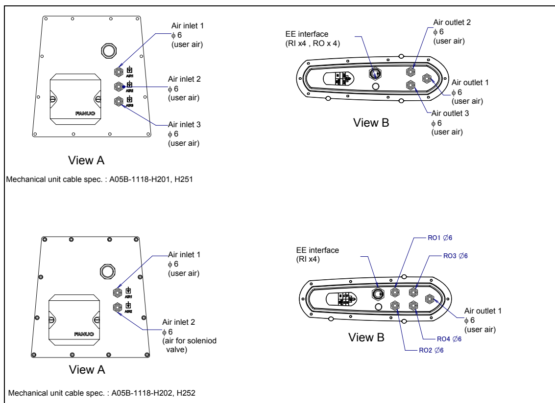
Fig. 5.2 (b) Air supply and EE (RI/RO) interface
