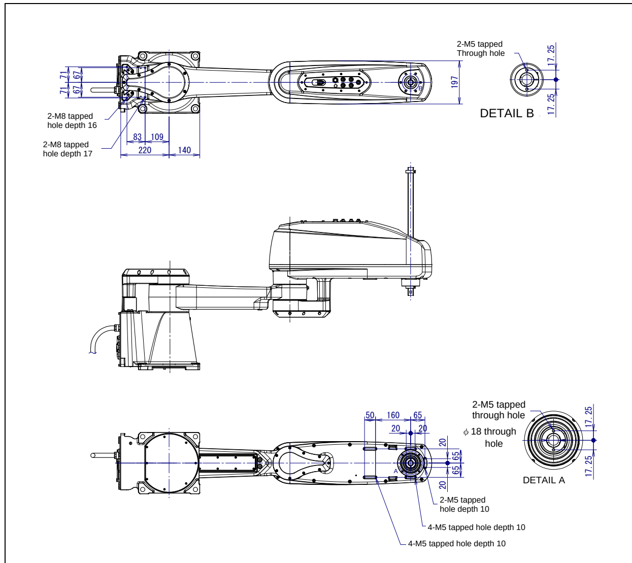
Fig. 4.2 (c) Equipment mounting faces (SR-20iA)
