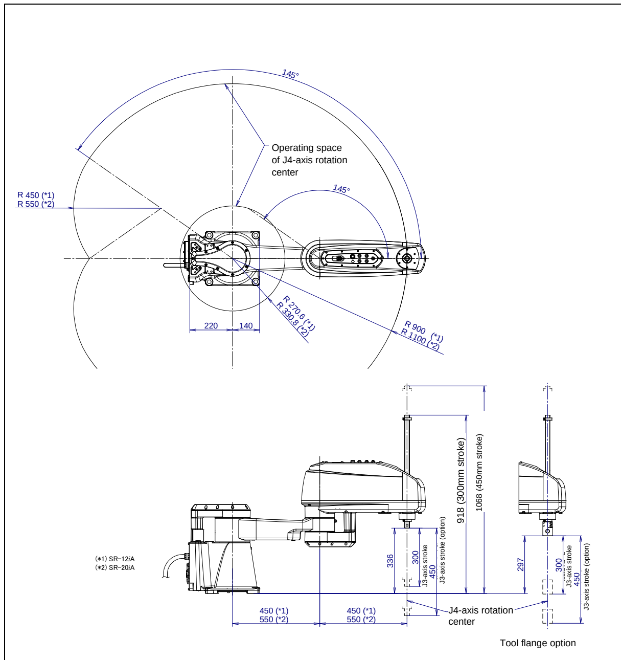
Fig. 3.2 (a) Operating space
