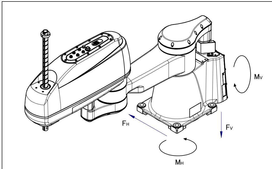
Fig. 1.2 (b) Force and moment that acts on J1 base
